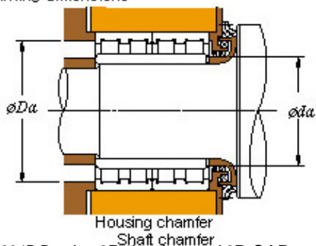
53FC37234B Bearing 2D drawings and 3D CAD models
